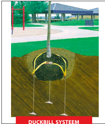
DUCKBILL SYSTEEM
